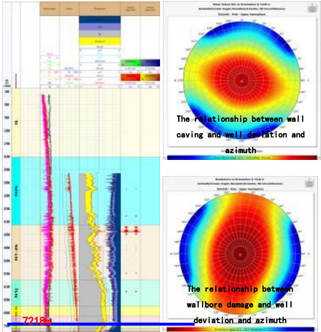
Geomechanical Analysis
